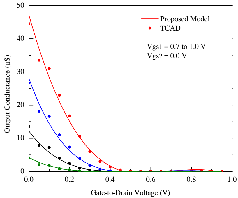
FIGURE 4.5: Comparison between modeled and simulated output characteristics of an independent gate FinFET with L_g = 100 nm.
