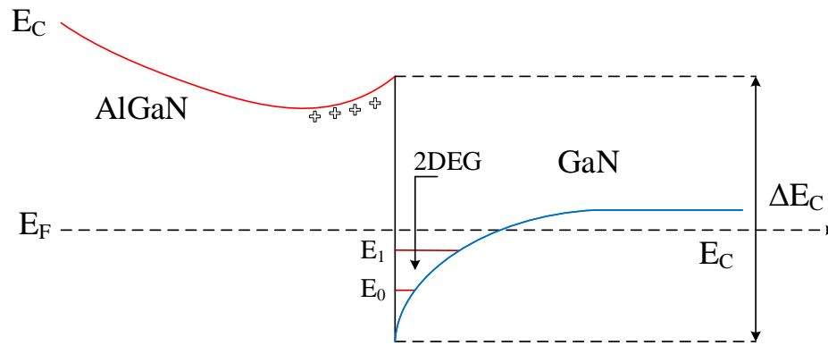
FIGURE 1.6: Difference in the bandgap energy of AlGaN and GaN resulting in the formation of 2DEG.
