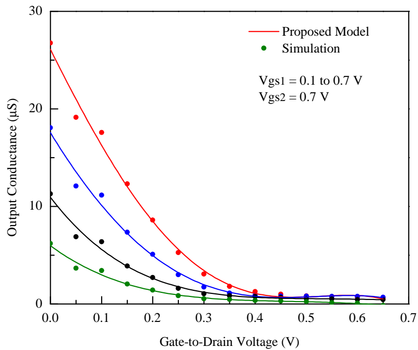
FIGURE 4.6: Comparison between modeled and simulated output characteristics of an independent gate FinFET with L_g = 10.8 nm.
