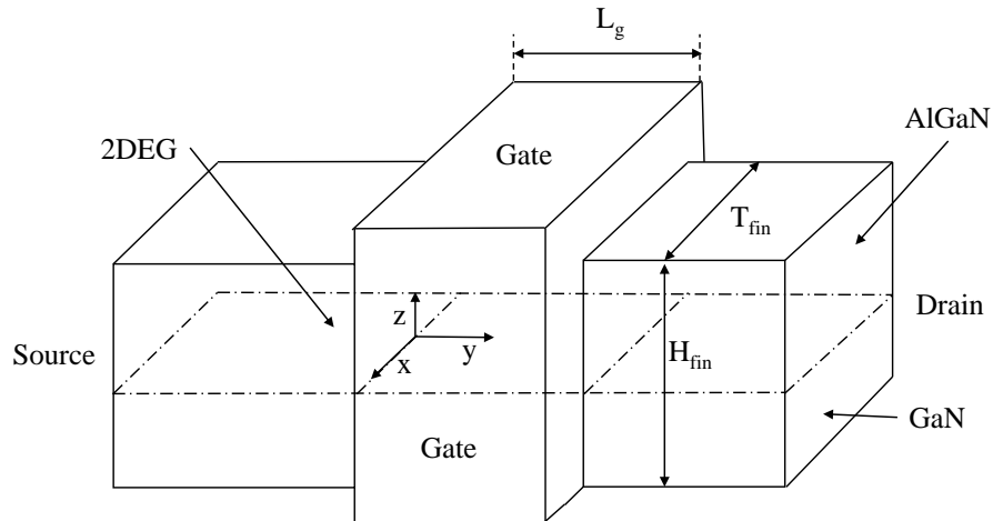
FIGURE 5.1: A view of AlGaN/GaN FinFET channel.
